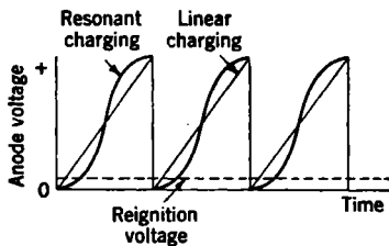
FIG. 8-46.—Anode-voltage waveforms for linear and resonant charging.
